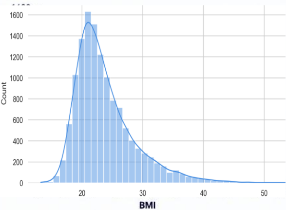
A. BMI DISTRIBUTION (HISTOGRAM)
